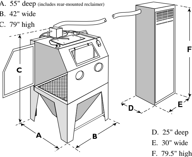
Model illustrated: BNP 65-600 DF 600 CFM Reclaimer (rear mounted) and Dry Filter
